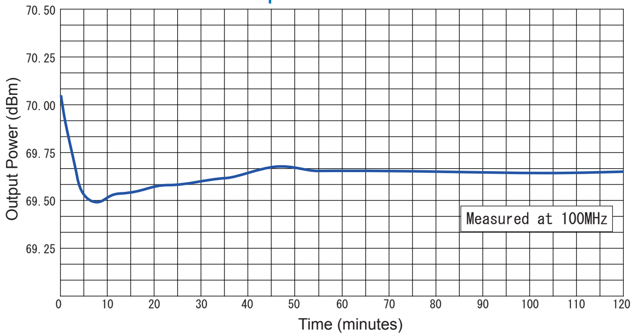
Output Power vs Time
