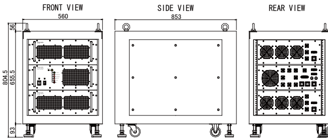
OUTLINE DRAWING
