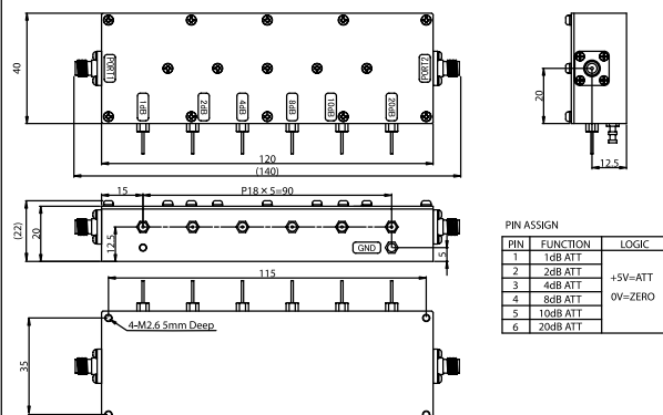
PT030-0S (Standard / SMA-FEMALE)
