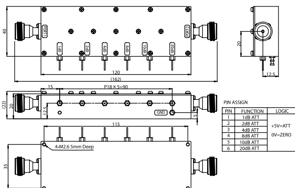
PT030-0N (Option / N-FEMALE)
