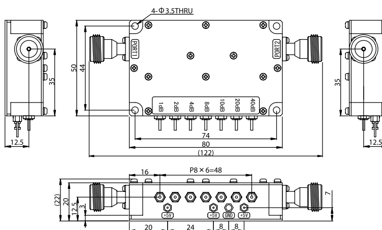
DT030-0N (Option / N-FEMALE)
