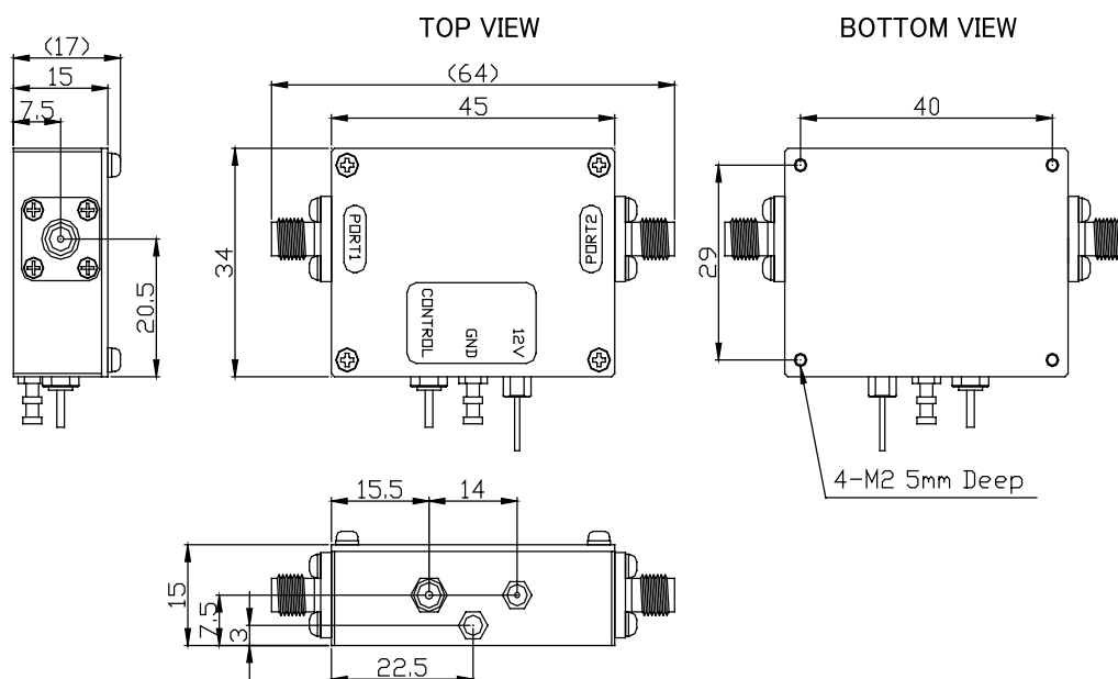
PI010-0S (Standard / SMA-FEMALE)
