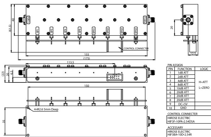
PT040-1S (Standard / SMA-FEMALE) (Option / TTL Drive)
