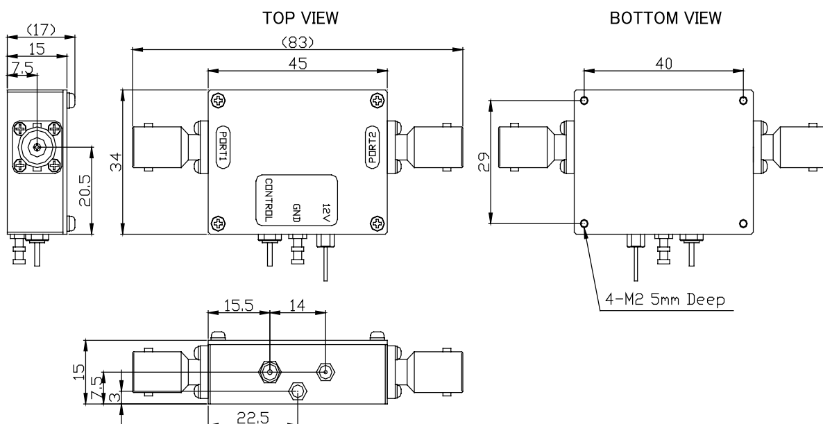
PI010-0B (Option / BNC-FEMALE)
