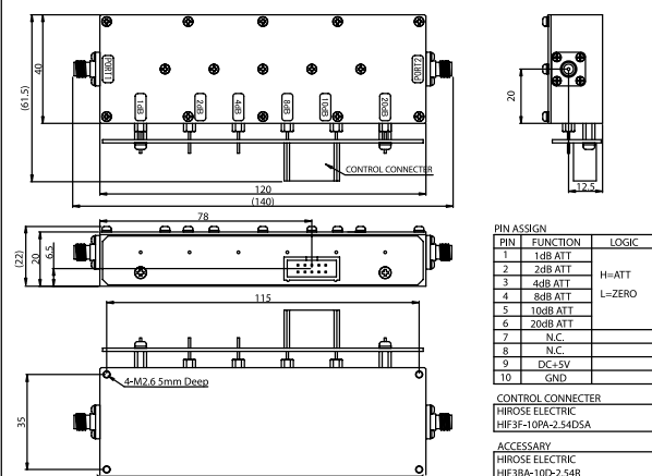
PT030-1S (Standard / SMA-FEMALE) (Option / TTL Drive)
