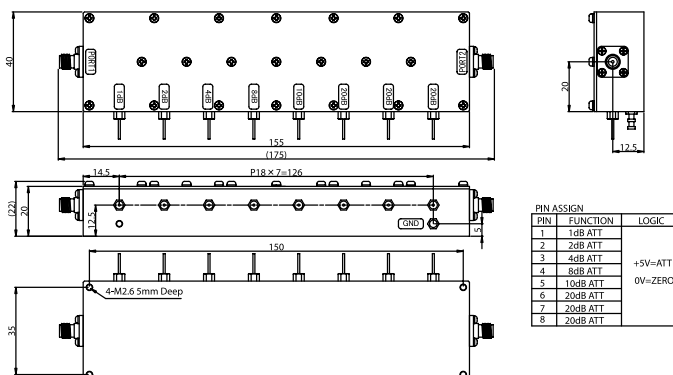
PT040-0S (Standard / SMA-FEMALE)
