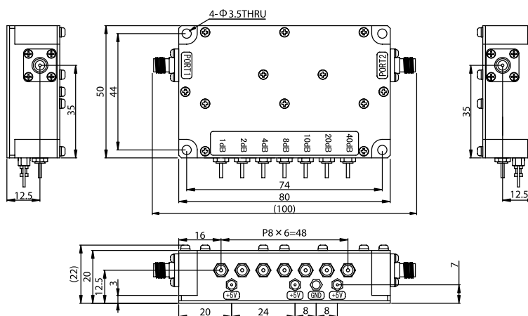
DT030-0B (Option / N-FEMALE)
