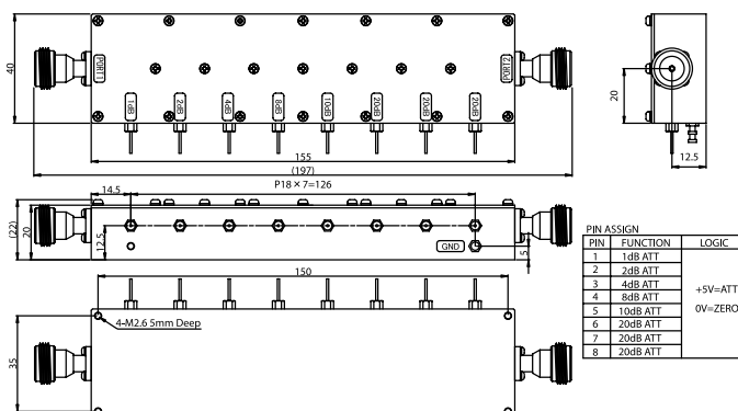
PT040-0N (Option / N-FEMALE)
