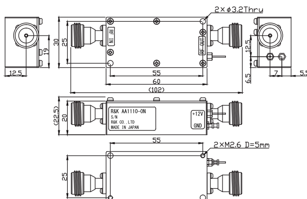
AA1110-0N (Option / N-FEMALE)
