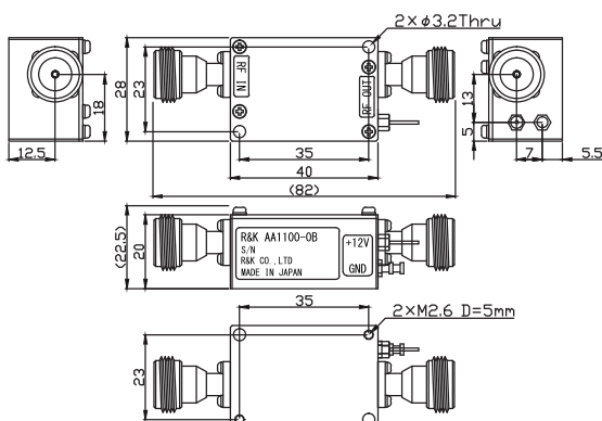
AA1100-0N (Option / N-FEMALE)
