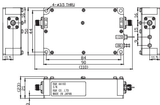
AA160-0S / AA180-0S AA290-0S / AA300-0S (Standard / SMA-FEMALE)
