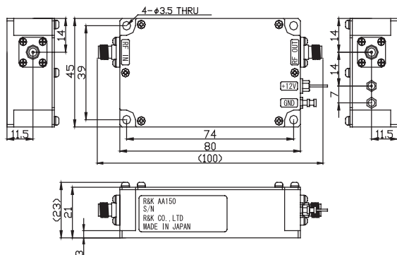
AA150-0S / AA170-0S (Standard / SMA-FEMALE)
