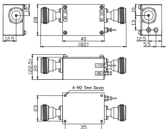
AA010-0N / AA050-0N AA270-0N / AA280-0N (Option / N-FEMALE)
