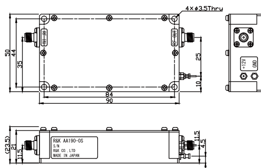
AA190-0S / AA200-0S (Standard / SMA-FEMALE)
