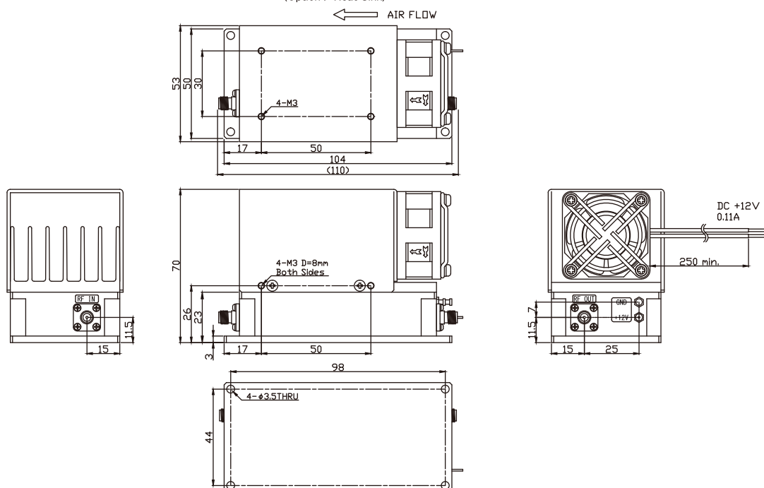
AA190-1S / AA200-1S (Standard / SMA-FEMALE) (Option / Heat Sink)
