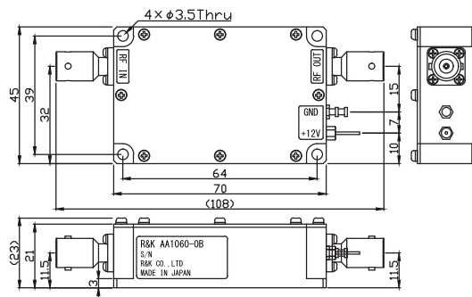
AA1060-0B / AA1080-0B (Option / BNC-FEMALE)
