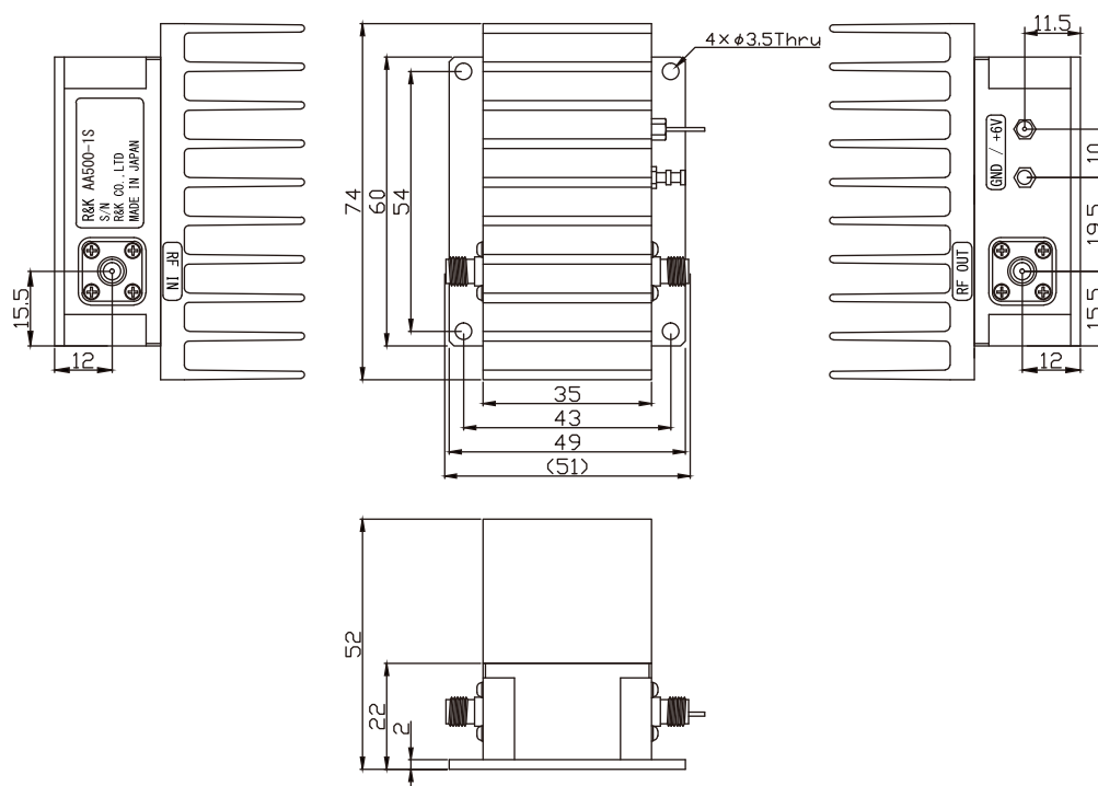
AA350-1S / AA360-1S / AA500-1S (Standard / SMA-FEMALE) (Option / Heat Sink)
