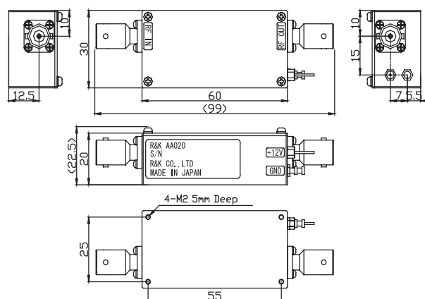
AA020-0N / AA060-0N (Option / N-FEMALE)
