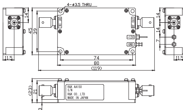
AA150-0B / AA170-0B (Option / BNC-FEMALE)
