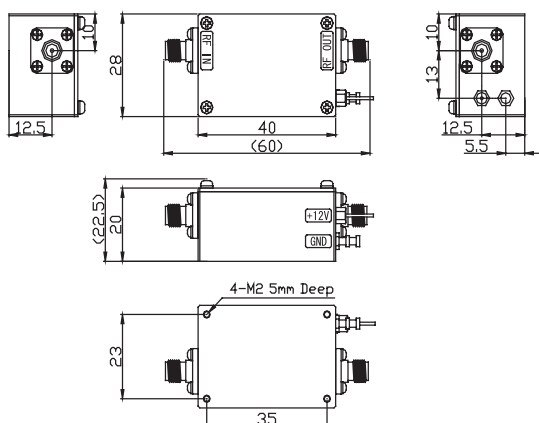
AA010-0S / AA050-0S AA270-0S / AA280-0S (Standard / SMA-FEMALE)
